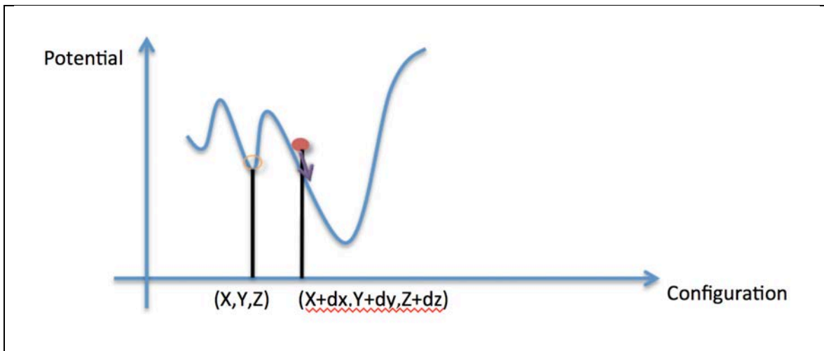
Figure 2.3. Potential surface scheme of an unstable crystal.
