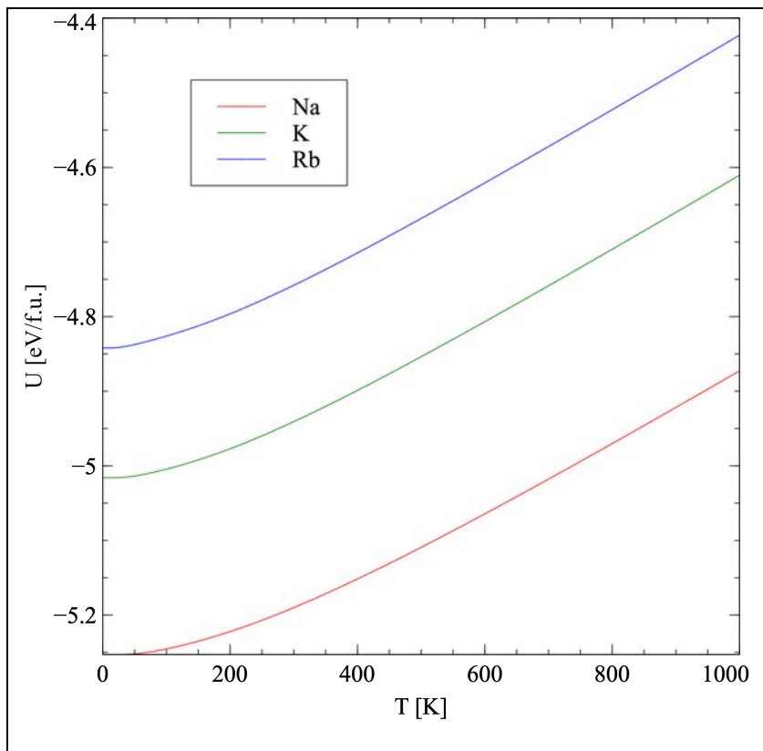
Figure 4.9. Theoretical internal energy of M\text{H}_{31}\text{OH} for M = \{\text{Na}, \text{K} \text{ and } \text{Rb}\} .
