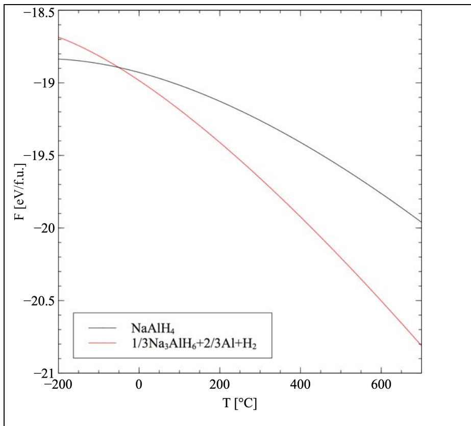
Figure 3.9. Comparison of theoretical free energies between \text{NaAlH}_4 and 1/3\text{Na}_3\text{AlH}_6+2/3\text{Al}+\text{H}_2 .
