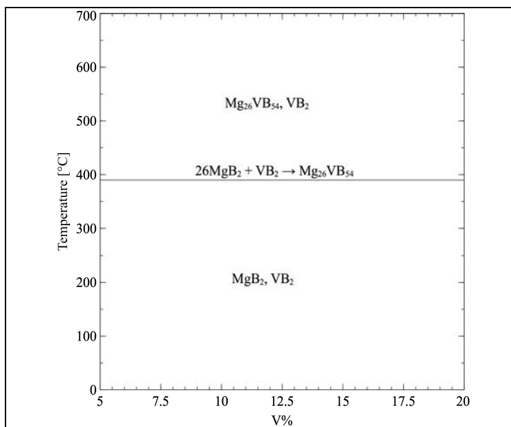
Figure 5.14. Theoretical phase diagram at Mg-rich side in Mg-V-B system.
