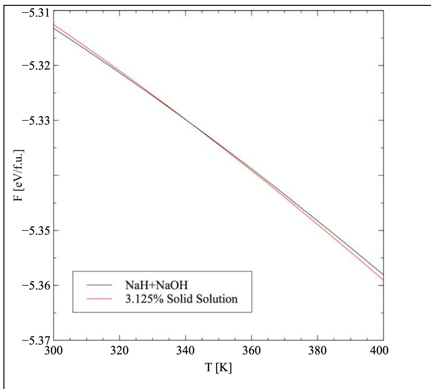
Figure 4.13. Comparison of theoretical free energies between \text{Na}_{32}\text{H}_{31}\text{OH} and 31\text{NaH}+\text{NaOH} .
