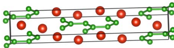
Figure 5.10. The crystal structure of V_2B_3 , V in red and B in green.
