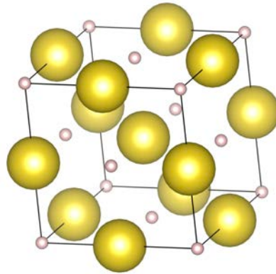
Figure 2.1. The crystal structure of NaH, Na in gold, H in white.
