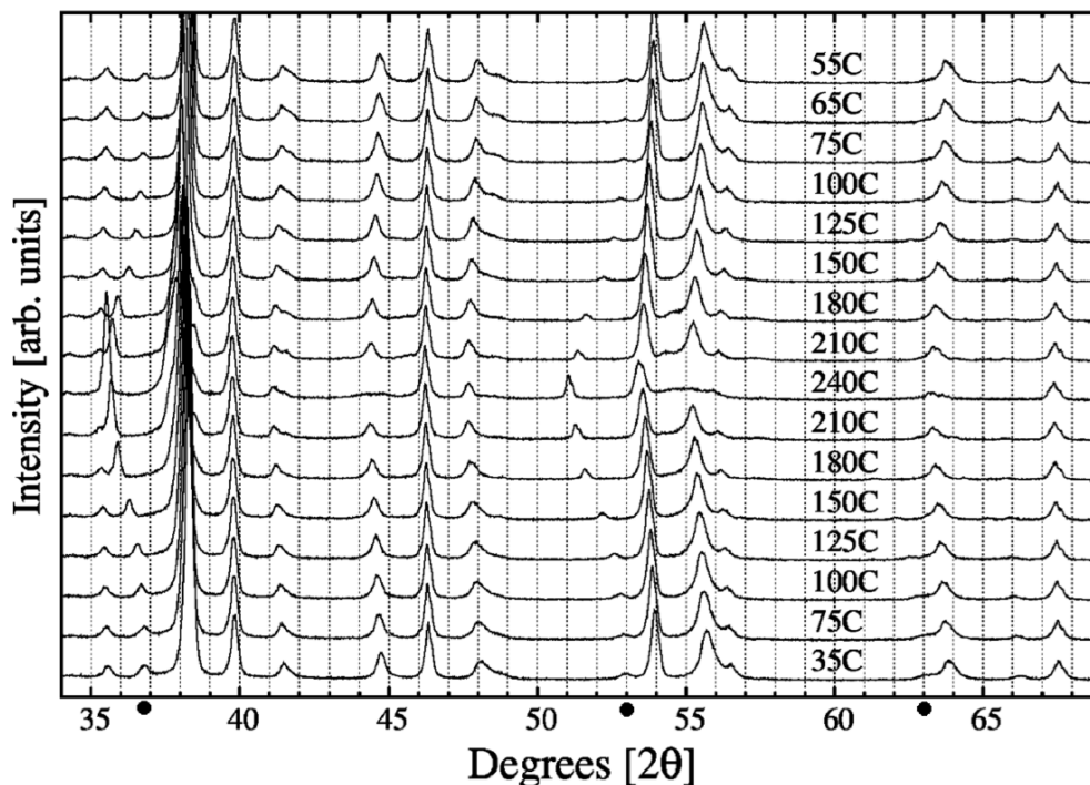
Figure 5. In situ XRD of 8:2 molar ratio of NaOH:NaH. Note the peak shifts of the NaH (200) at about 37° and (220) at about 53° (highlighted by black dots on the x-axis); the weak (311) at about 63° shifts similarly but is only evident with magnification. Refer to Figure 4 for identification of the peaks. Vertical guidelines (dotted lines) are given to emphasize the peak shifts.
