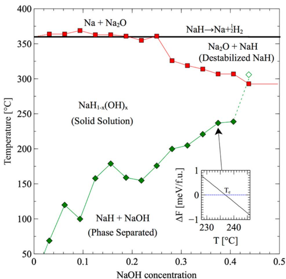
Figure 2. Critical temperatures for mixing and decompositions in the NaH/NaOH system: green, critical temperature; red, decomposition of solid solution; black, decomposition of NaH at P = 1 bar of \text{H}_2 . Inset illustrates critical temperature.
