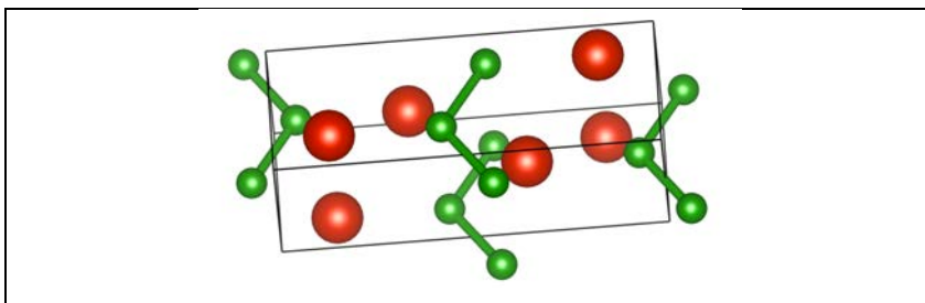
Figure 5.13. The crystal structure of VB, V in red and B in green.
