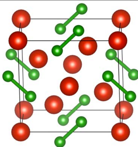
Figure 5.11. The crystal structure of V_3B_2 , V in red and B in green.
