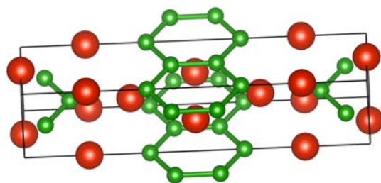
Figure 5.12. The crystal structure of V_3B_4 , V in red and B in green.
