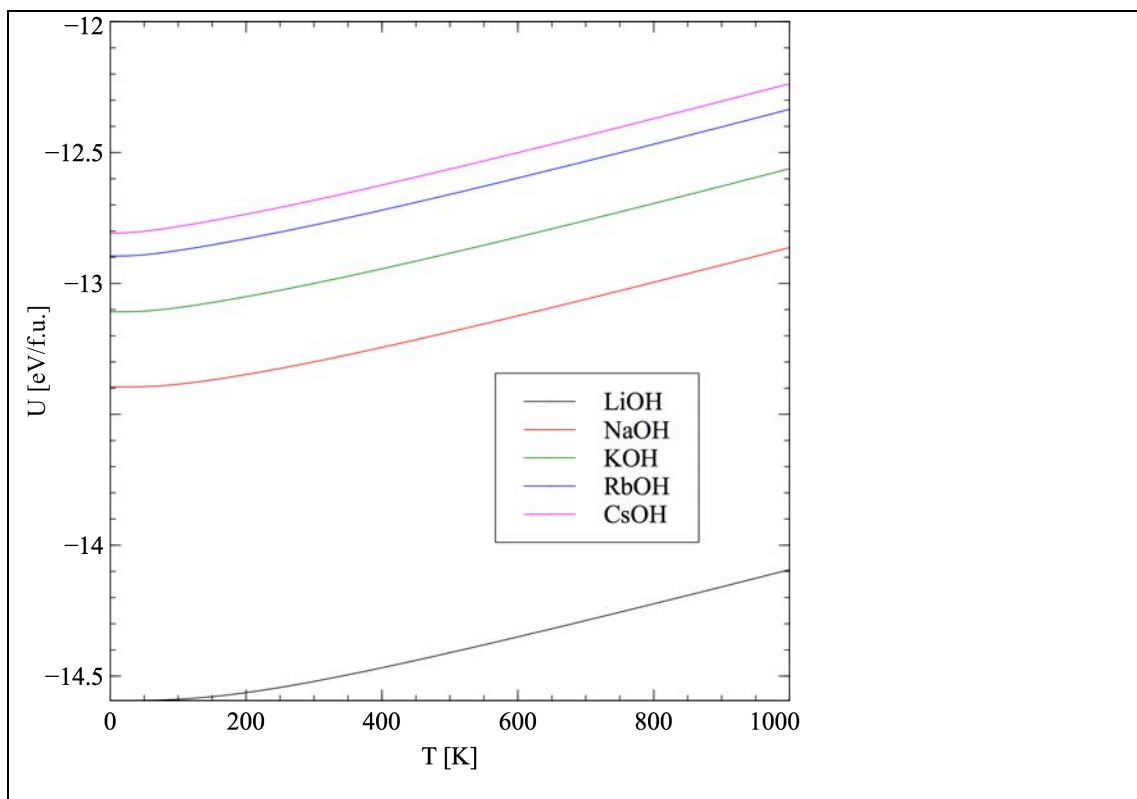
Figure 4.6. Theoretical internal energy of alkali metal hydroxides as a function of temperature.
