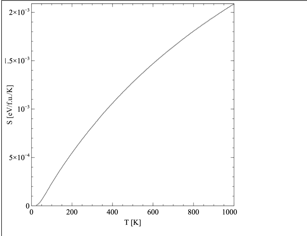
Figure 3.4. Theoretical entropy of NaAlH 4 as a function of temperature.
