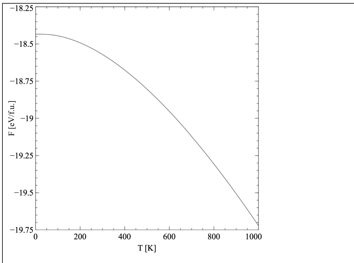
Figure 3.13. Theoretical free energy of (\text{NaAlH}_4)_{15}\text{NaOH} as a function of temperature.
