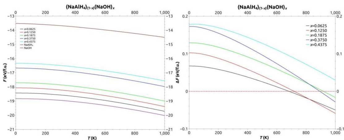
Figure 5 (Left). The free energies of (\text{NaAlH}_4)_{(1-x)}(\text{NaOH})_x . (Right). The changes of free energies. For a particular concentration x , OH - is soluble when \Delta F < 0 . As x increases \Delta F at 0 K also increases.
