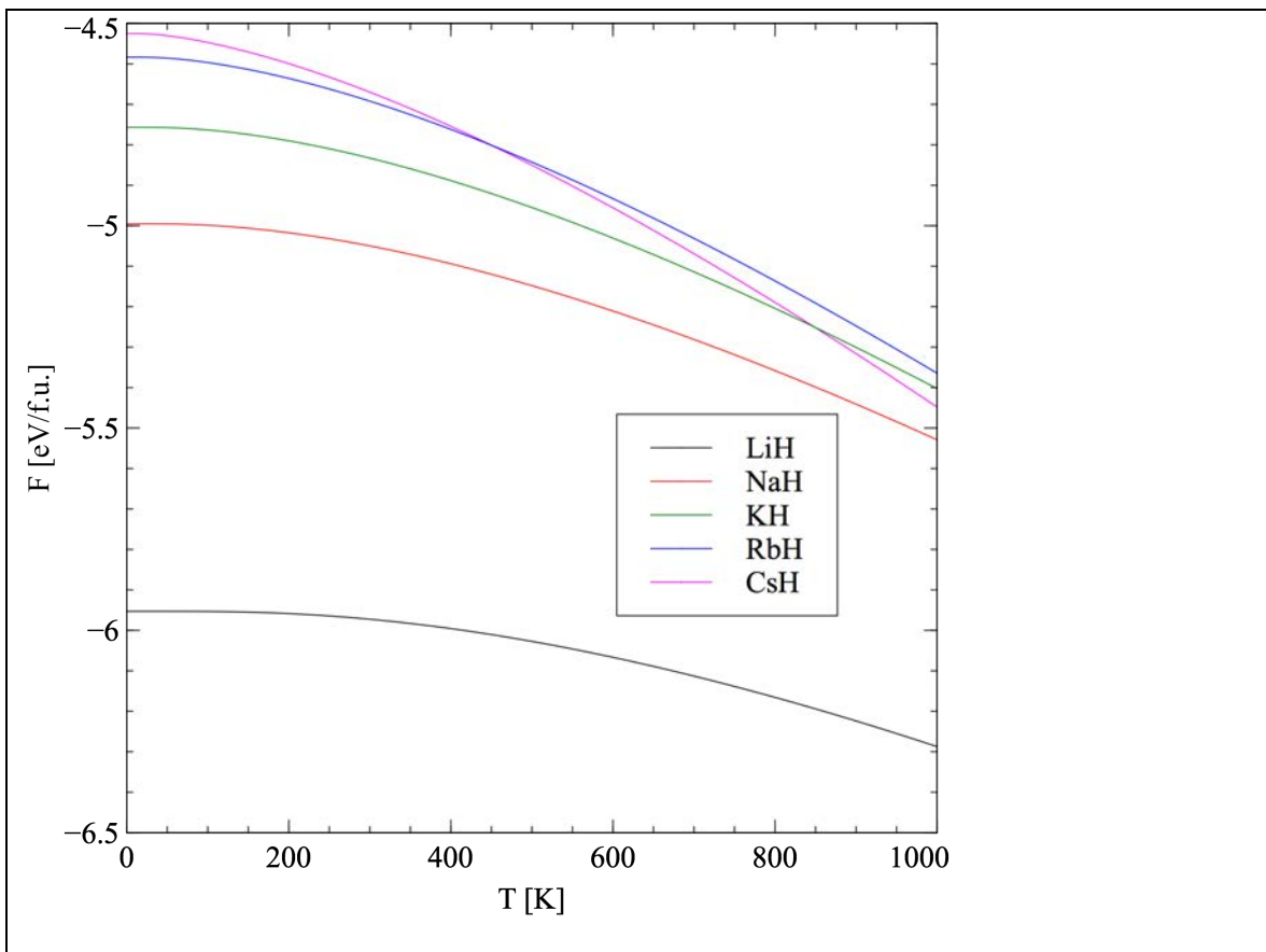
Figure 4.4. Theoretical free energy of alkali metal hydrides as a function of temperature.
