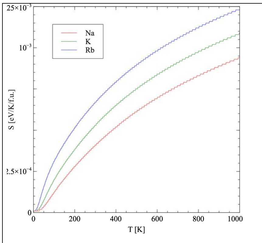
Figure 4.11. Theoretical entropy of MH_{31}OH for M = \{Na, K and Rb\} .
