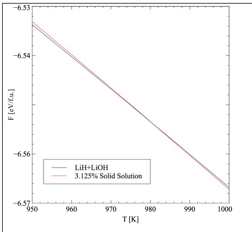
Figure 4.12. Comparison of theoretical free energies between \text{Li}_{32}\text{H}_{31}\text{OH} and 31\text{LiH}+\text{LiOH} .
