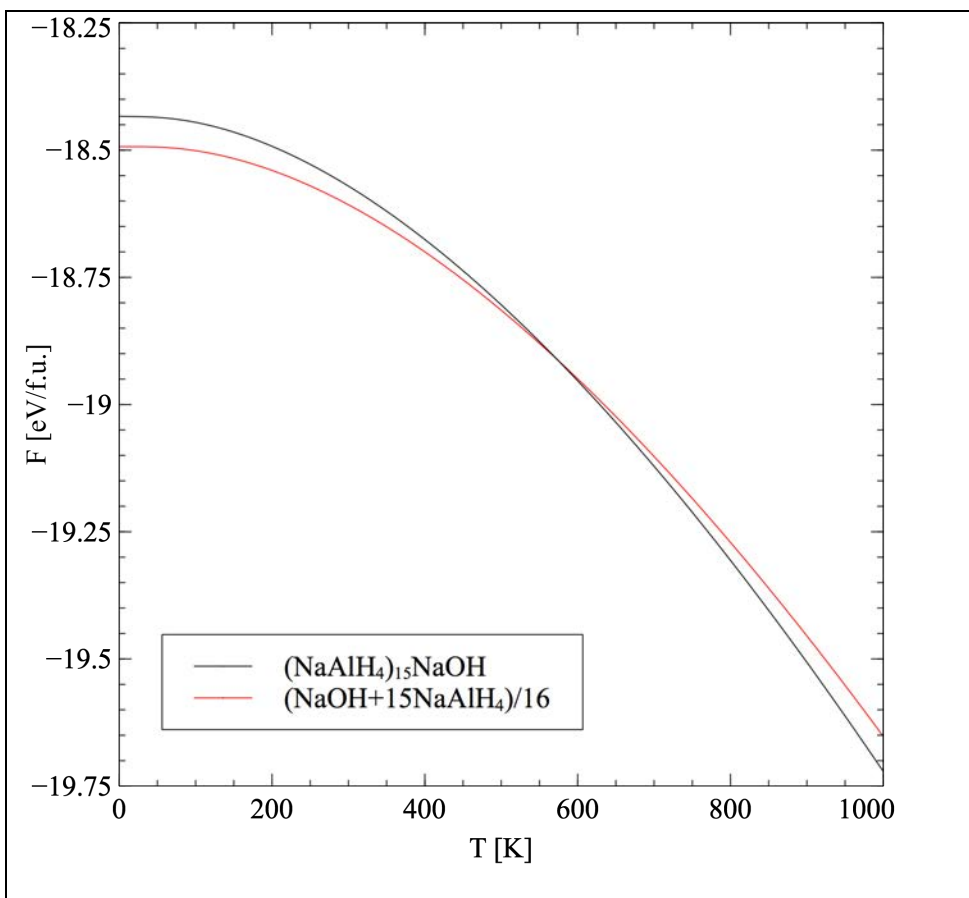
Figure 3.14. Comparison of theoretical free energies between (\text{NaAlH}_4)_{15}\text{NaOH} and \text{NaAlH}_4 + \text{NaOH} .
