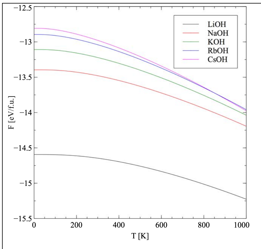
Figure 4.7. Theoretical free energy of alkali metal hydroxides as a function of temperature.
