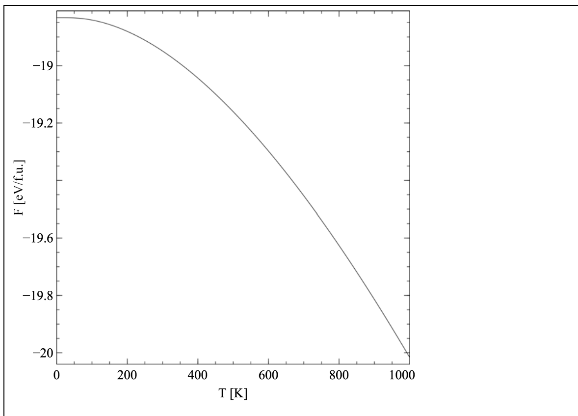
Figure 3.3. Theoretical free energy of \text{NaAlH}_4 as a function of temperature.
