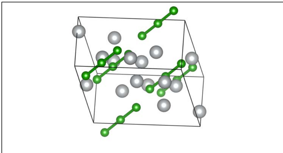
Figure 5.27. The crystal structure of Ni_4B_3 , Ni in grey and B in green.
